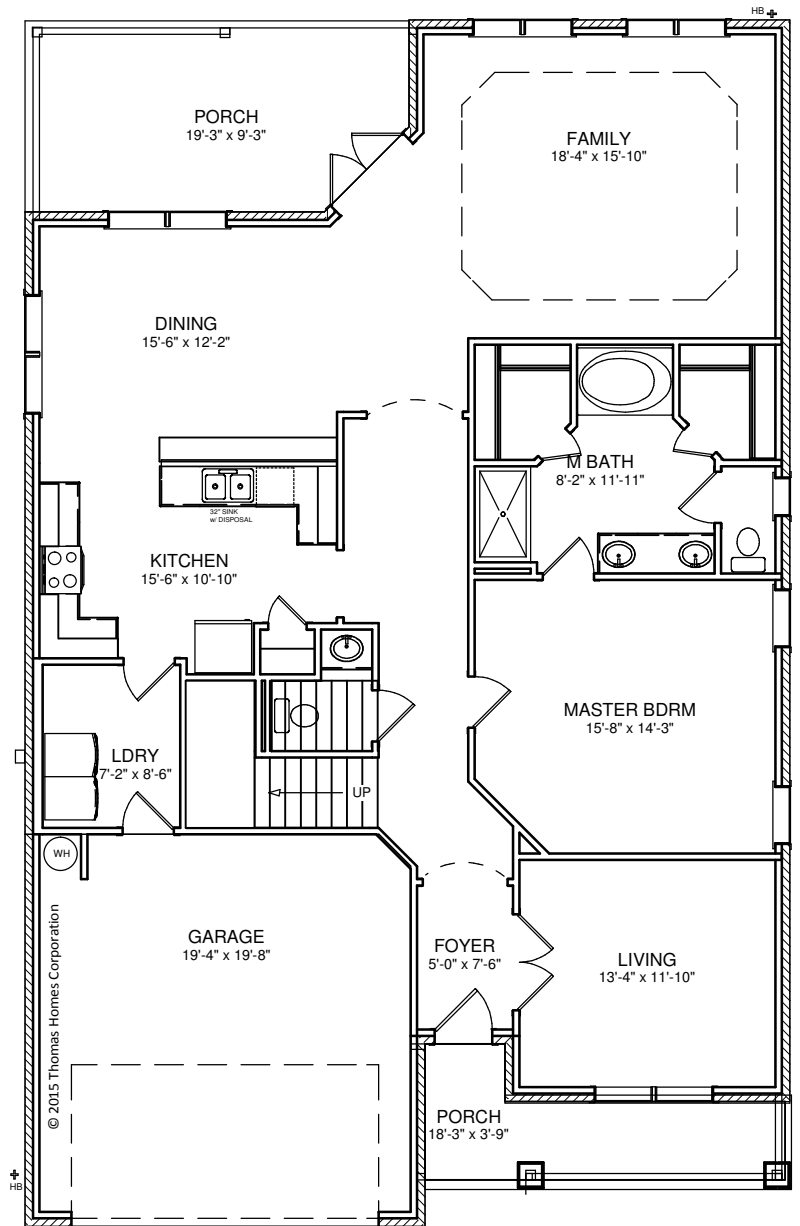
1st Floor
