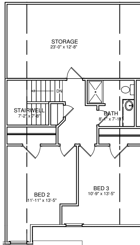
2nd Floor
